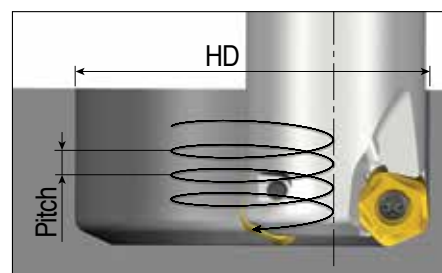
Helical ramping
