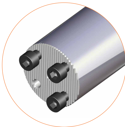
Serrated coupling design
